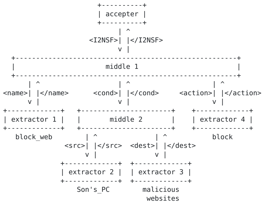
Figure 3: The Example of High-level Policy
