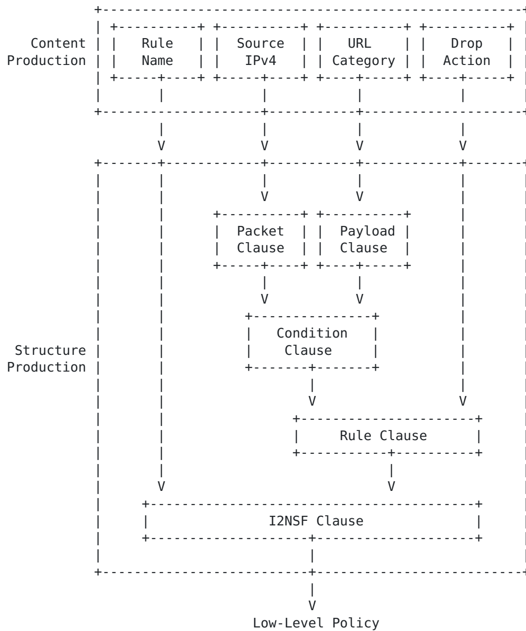
Figure 9: Generator Construction for Web-Filter NSF
