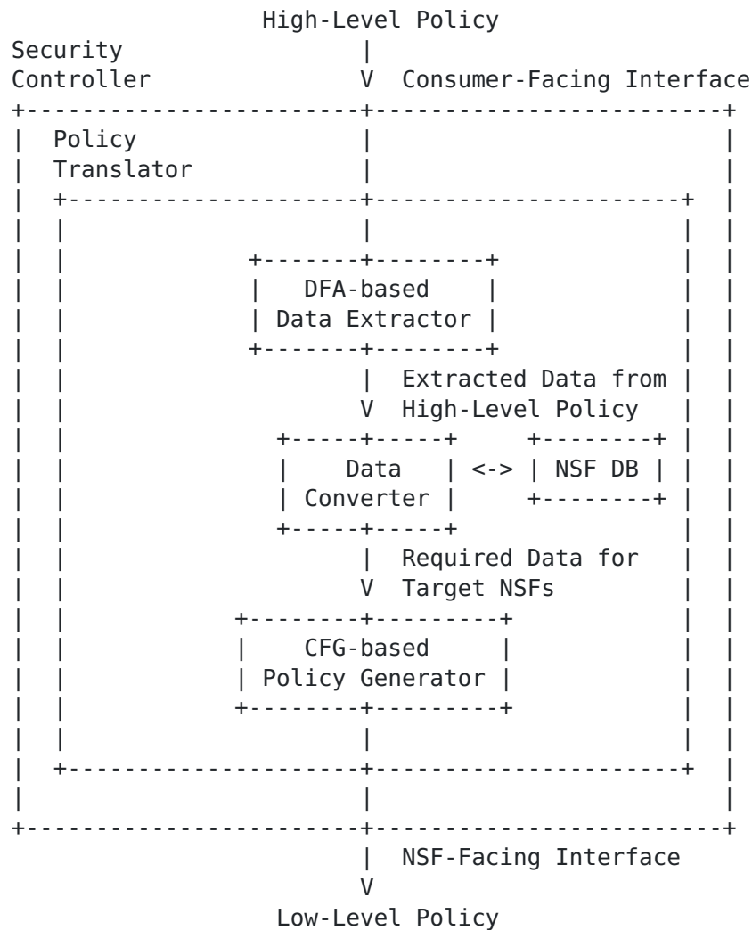
Figure 1: The Overall Design of Policy Translator
