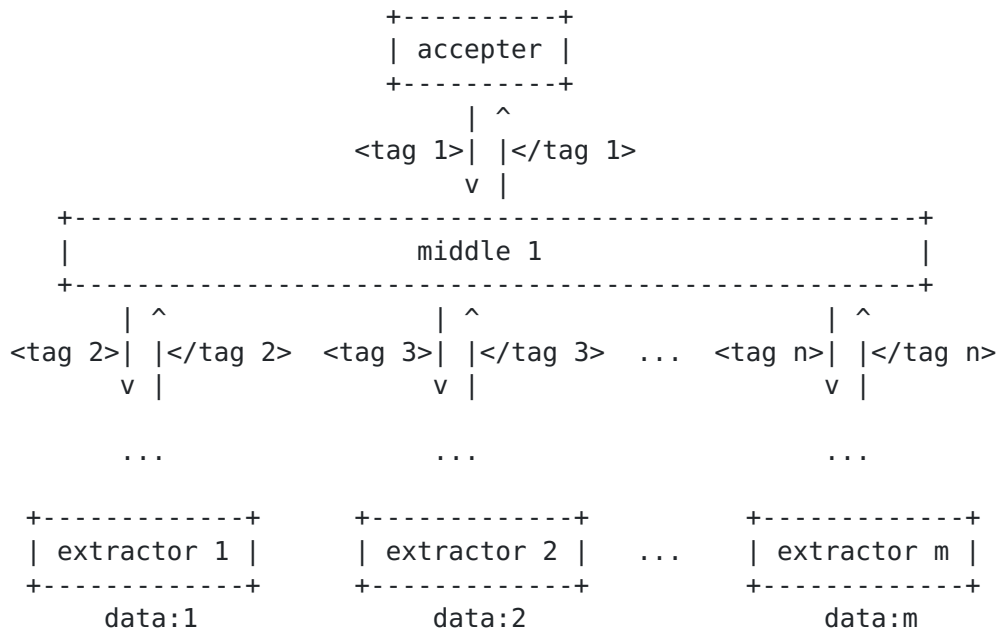
Figure 2: DFA Architecture of Data Extractor
