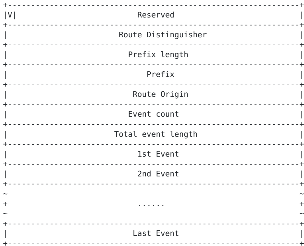
Figure 1: Route Policy and Attribute Trace Message format
