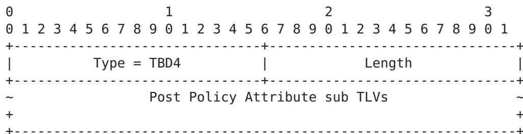
Figure 7: Post Policy Attribute TLV
