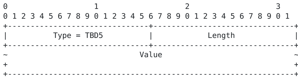
Figure 8: String TLV
