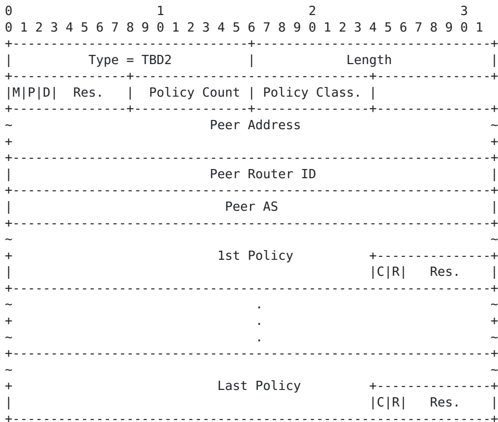
Figure 4: Policy TLV
