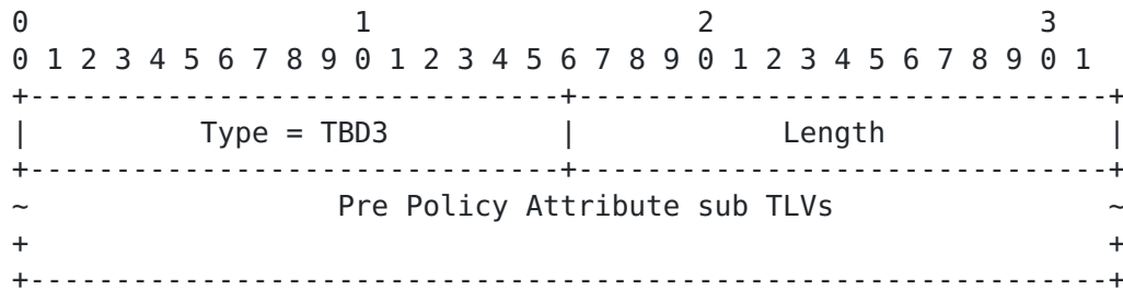
Figure 6: Pre Policy Attribute TLV
