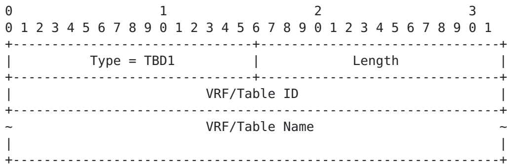
Figure 3: VRF/Table TLV
