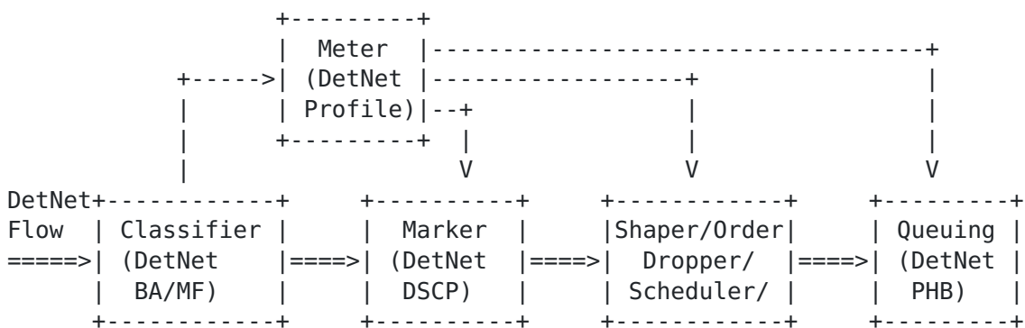
Figure 1: Overview of a DetNet DiffServ mechanism
