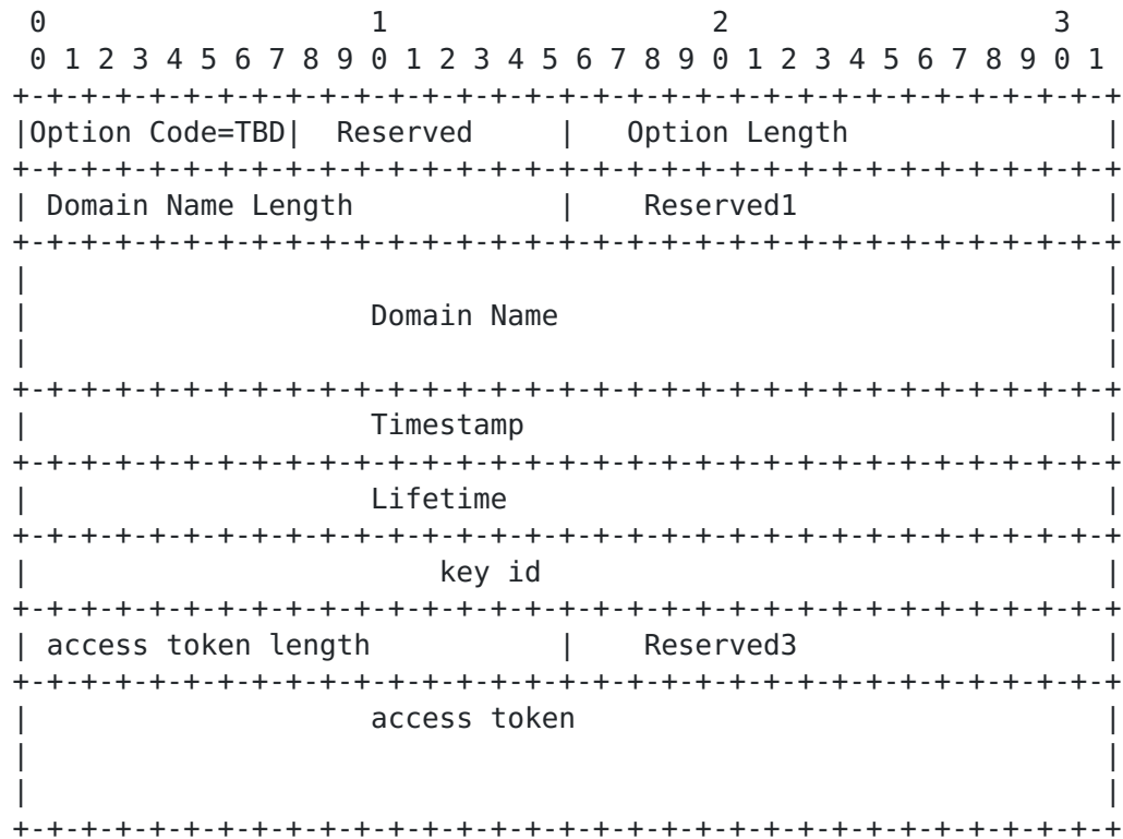
Figure 4: PCP ACCESS_TOKEN Option
