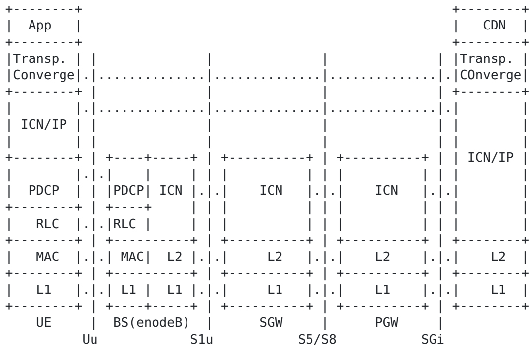
Fig. 8. Native ICN Deployment in UE
