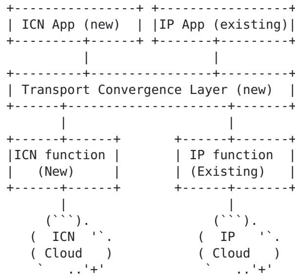
Fig. 4. IP/ICN Convergence and Deployment Scenarios
