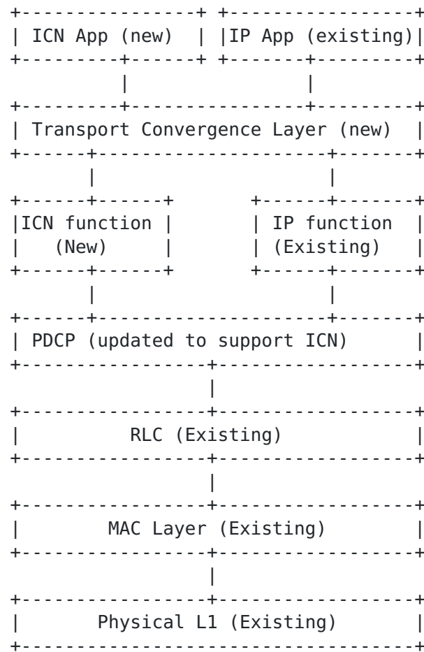
Fig. 7. Dual stack ICN protocol interactions
