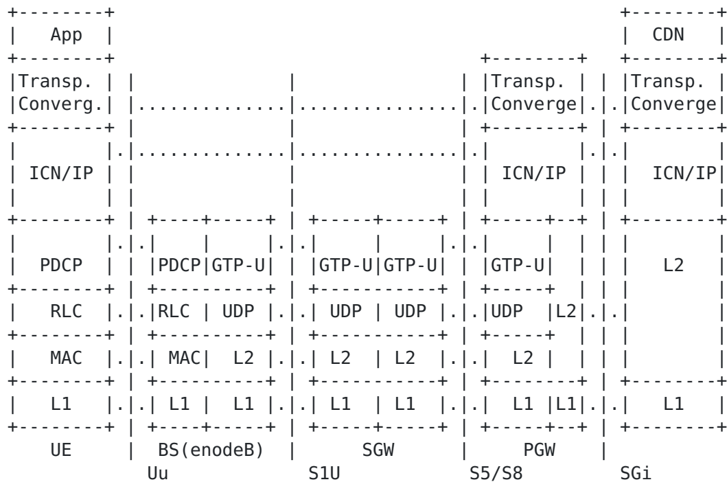
Fig. 6. Dual stack ICN Deployment in UE
