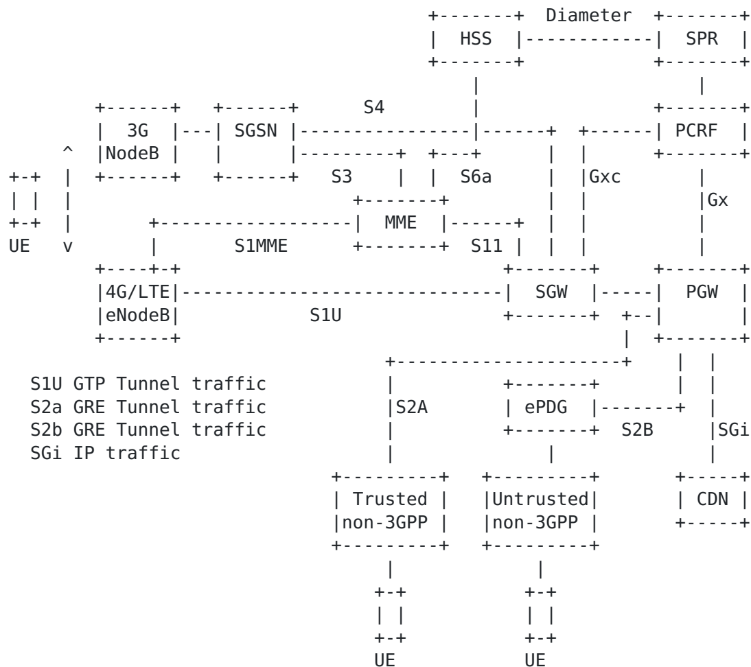
Figure-1: LTE, 4G Mobile Network Overview
