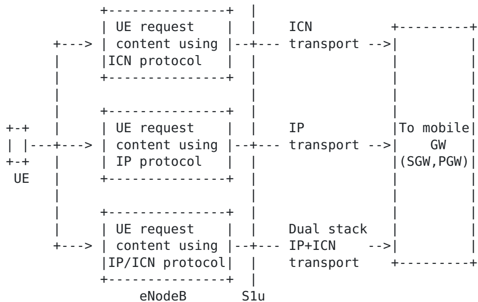
Fig. 9. Native ICN Deployment in eNodeB
