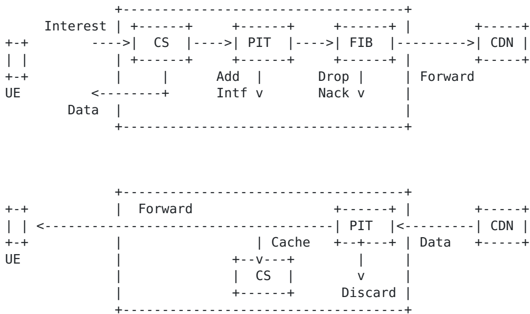
Fig. 3. ICN Interest, Data Packet and Forwarder
