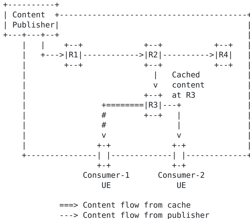
Fig. 2. ICN Architecture
