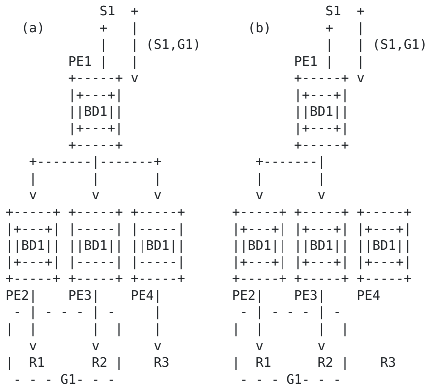
Figure 1 - Intra-subnet IP Multicast
