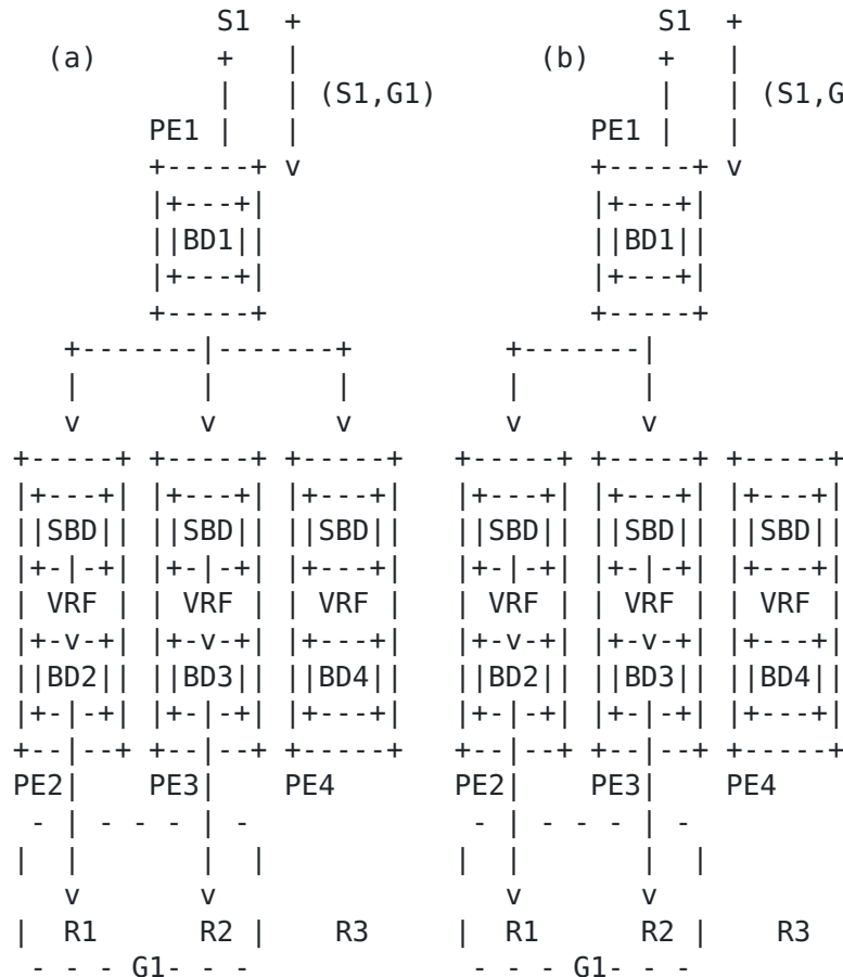
Figure 2 - Inter-subnet IP Multicast
