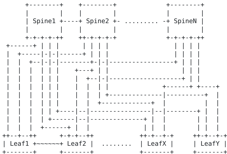
Figure 1: A Spine-Leaf Topology
