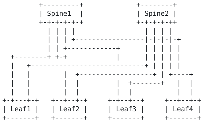
Figure 2: A CLOS Topology
