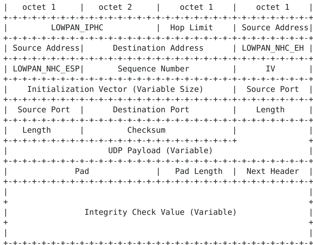
Figure 4: A sample NHC compressed IP/UDP packet secured with ESP.
