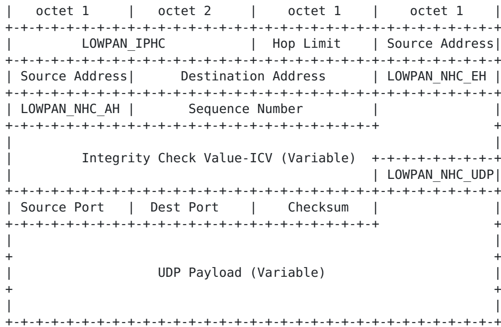
Figure 2: A sample NHC compressed IP/UDP packet secured with AH.
