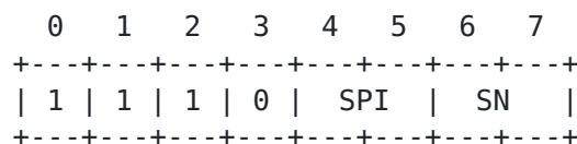
Figure 3: Proposed LOWPAN NHC encoding for ESP
