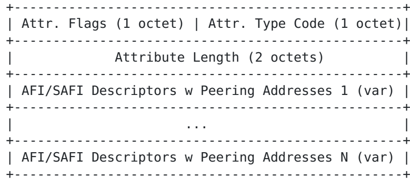
Figure 1: BGP Peer Discovery Attribute
