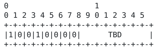
Figure 2: Flags & Type Code Fields
