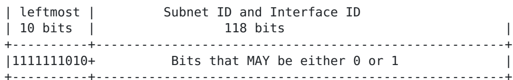
Figure 1: The IPv6 link-local address
