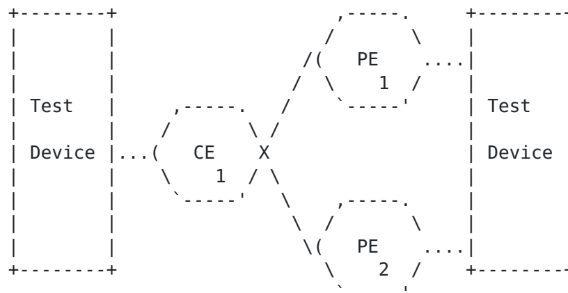
Figure 1 SUT for Throughput and other Ethernet Segment Tests
