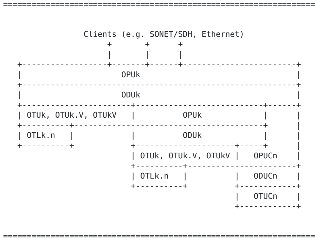
Figure 3: Digital Structure of OTN interfaces (from G.709:Figure 6-1)
