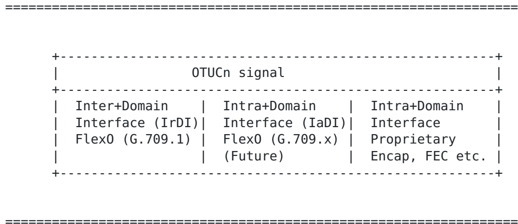
Figure 1: OTUCn transport possibilities
