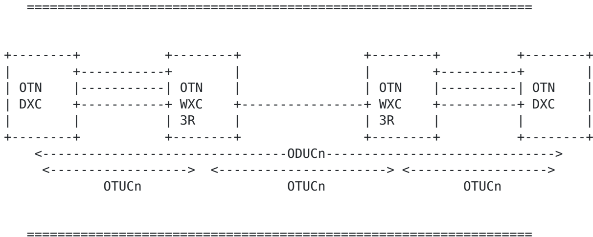
Figure 2: ODUCn signal
