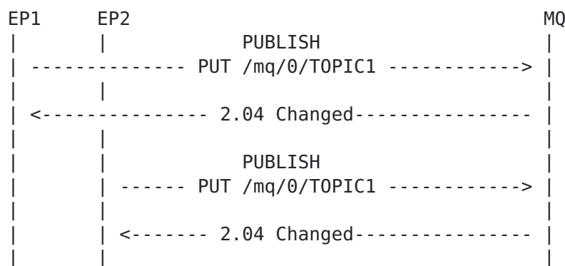
Figure 10: Multiple CoAP-MQ EPs PUBLISH to Broker
