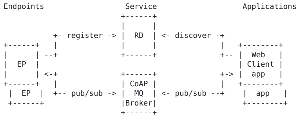
Figure 1: CoAP MQ Architecture
