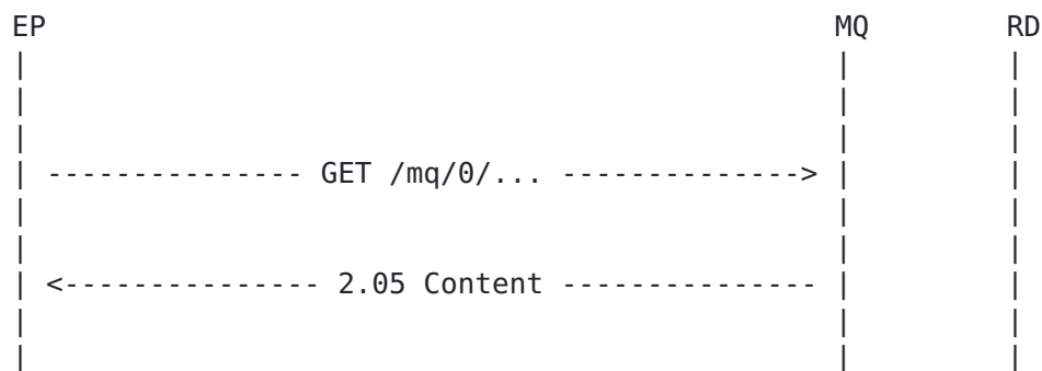
Figure 6: Client EP GET from CoAP-MQ Broker
