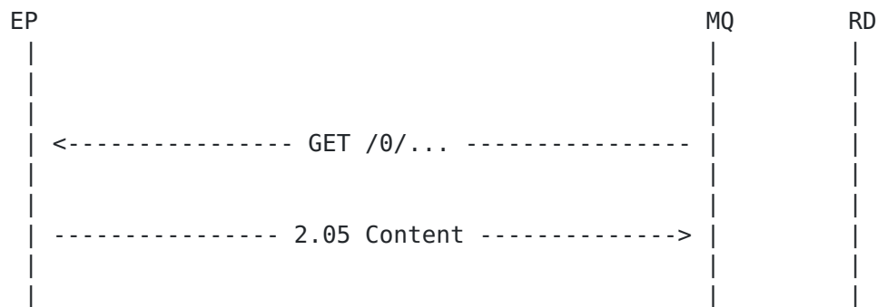
Figure 9: Broker GET from Server Role Endpoint
