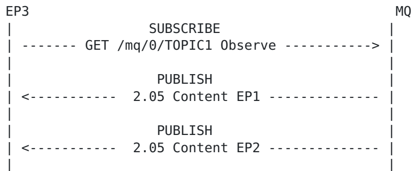
Figure 11: CoAP-MQ Endpoint SUBSCRIBE to Broker
