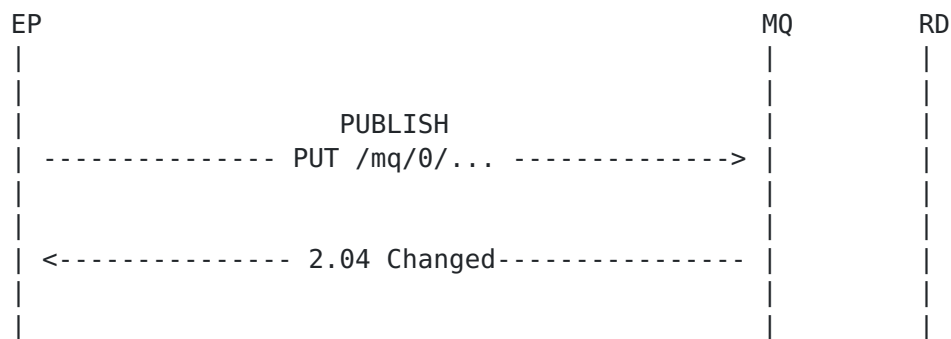
Figure 4: Client Role PUBLISH from EP to Broker
