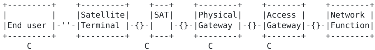
Figure 6: Network architecture for dealing with LAN losses
