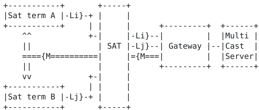
Figure 4: Network architecture for a reliable multicast with NC
