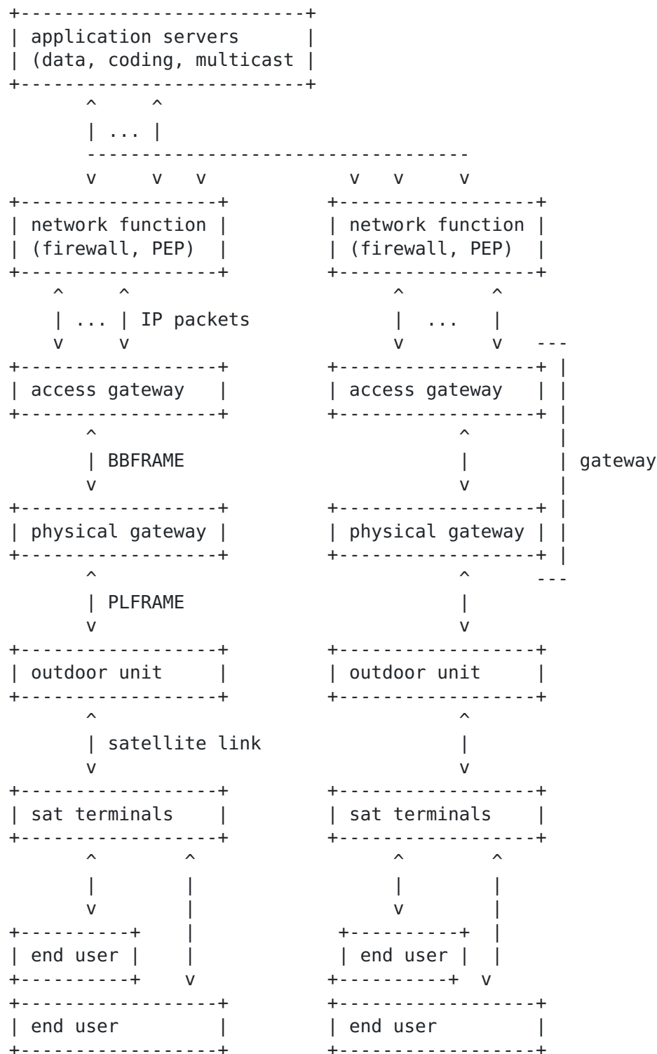
Figure 2: Data plane functions in a generic satellite multi-gateway system
