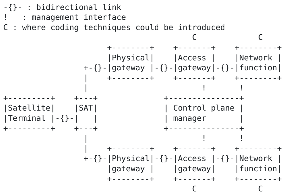
Figure 8: Network architecture for dealing with gateway handover schemes
