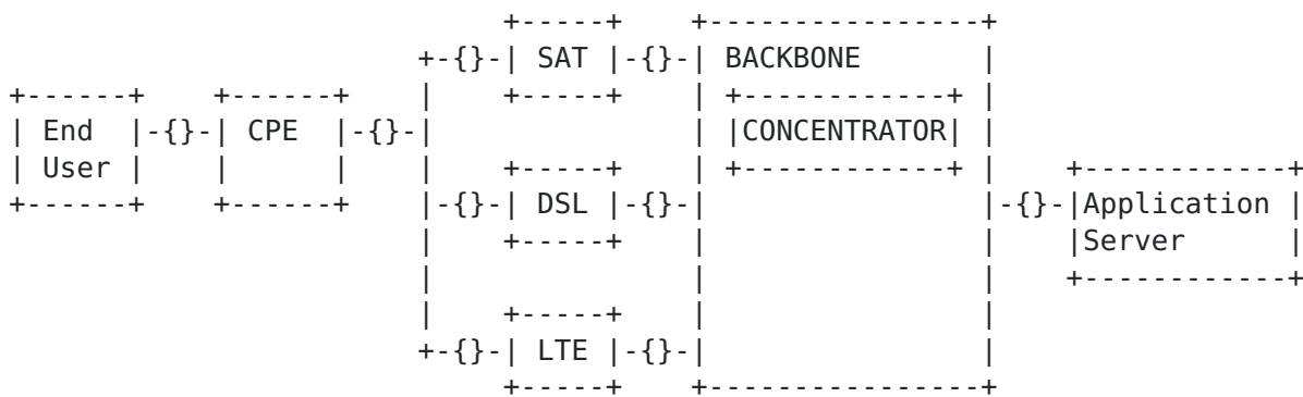
Figure 5: Network architecture for an hybrid access using coding
