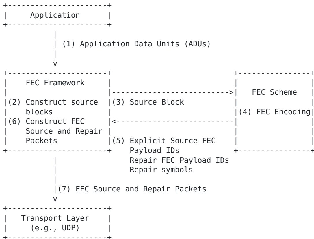
Figure 1: FECFRAME architecture at a sender.
