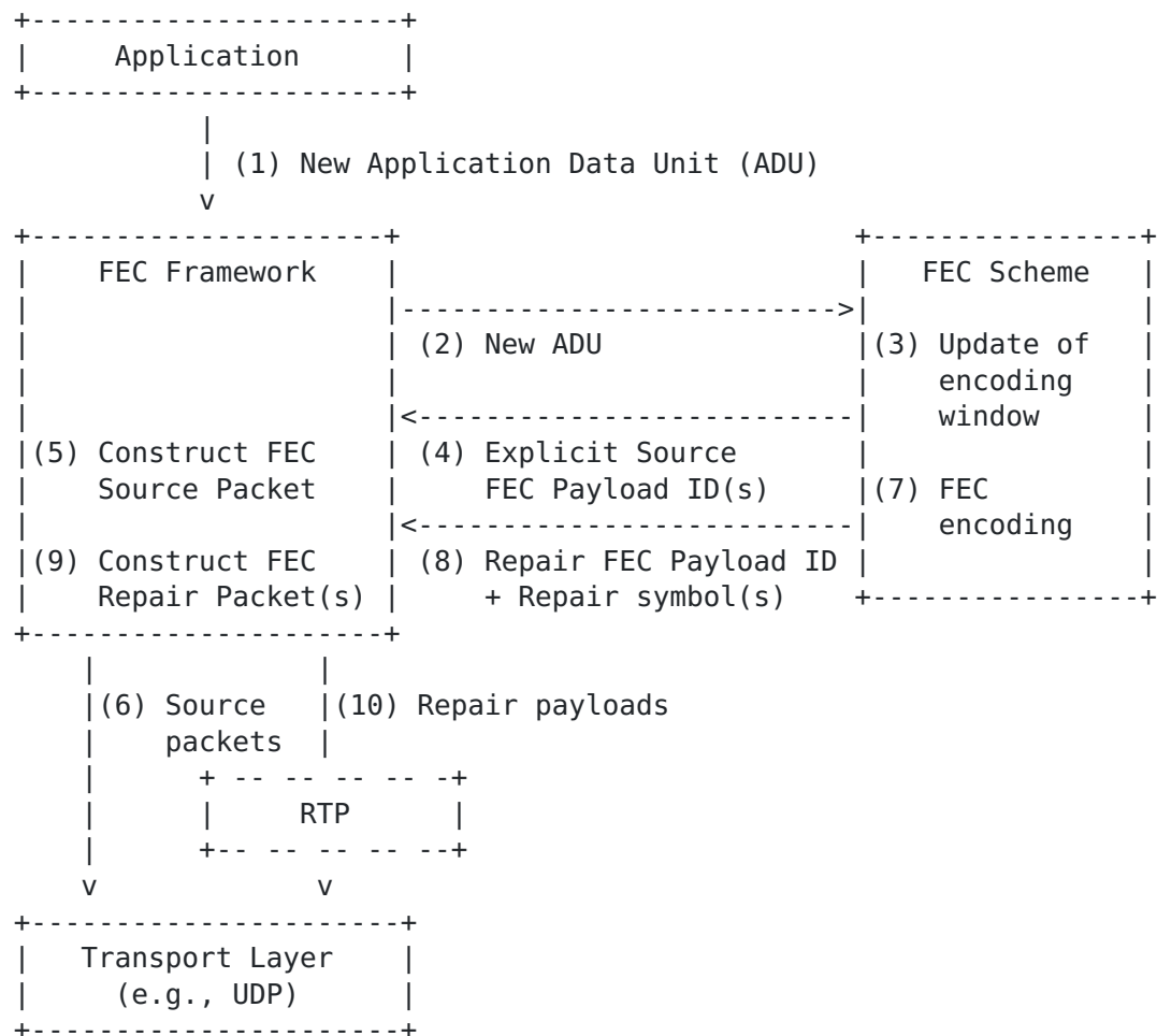
Figure 3: Sender Operation with RTP Repair Flows
