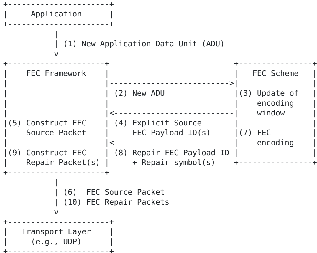
Figure 2: Sender Operation with Sliding Window FEC Codes
