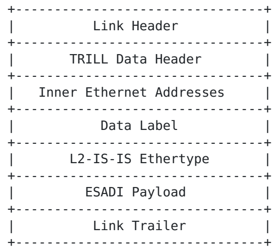
Figure 1. TRILL ESADI Packet Overview
