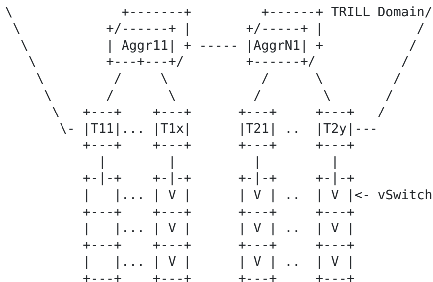
Figure 1. TRILL domain in typical Data Center Network
