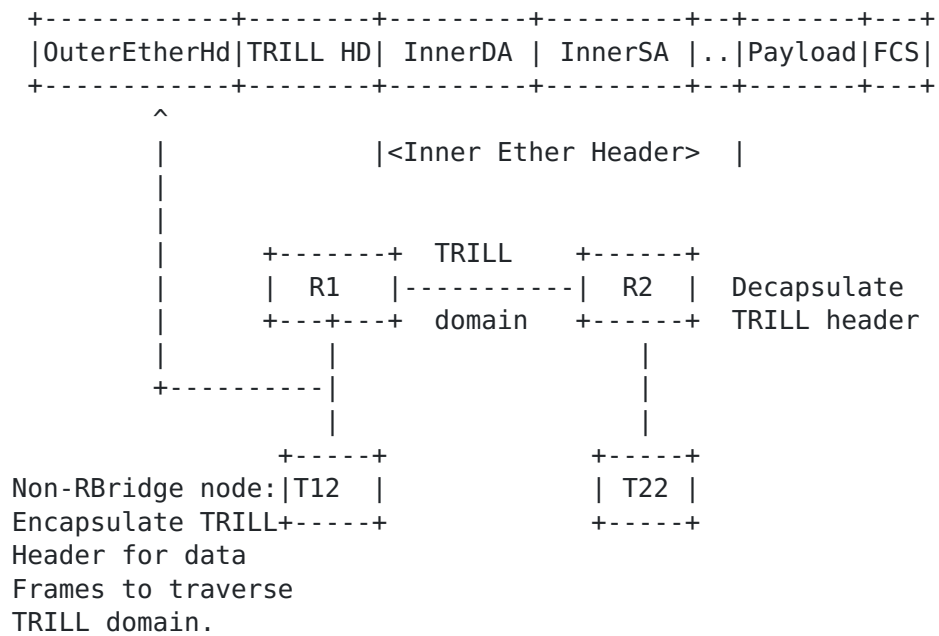
Figure 2. Data frames from TRILL-EN
