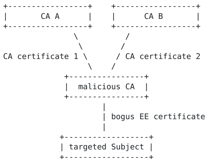
Figure 2: Multiple Certificate Chains for a Bogus Certificate
