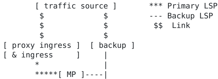
Figure 2: Example Protected LSP with Proxy Ingress Node
