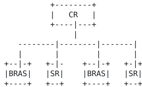
Fig.2 Star-mode Network Topology within MAN
