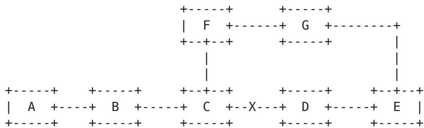
Figure 3: Resource Sharing in 1+R Recovery Scheme
