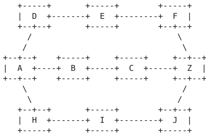
Figure 2: An Example of 1+1+R Recovery Scheme
