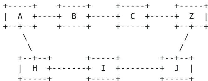
Figure 1: An Example of 1+R Recovery Scheme
