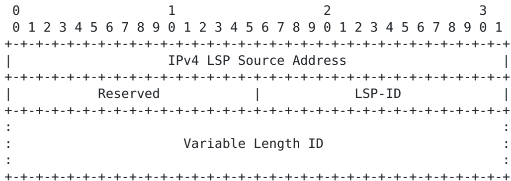
Figure 4: IPv4 Extended Association ID Format Example
