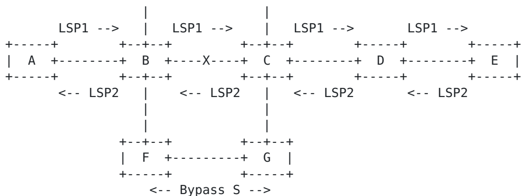
Figure 1: Multiple Bidirectional Bypass Tunnels
