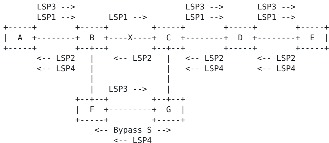
Figure 3: Restoration LSP Set-up after Link Failure
