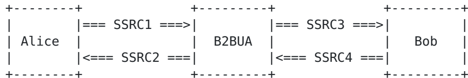
Figure 1: B2BUA modifying RTP headers
