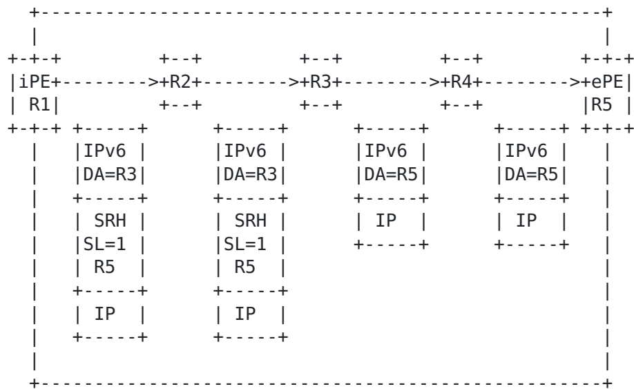
Figure 1: PSP use-case topology
