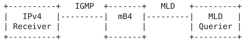
Figure 2: IGMP-MLD Interworking
