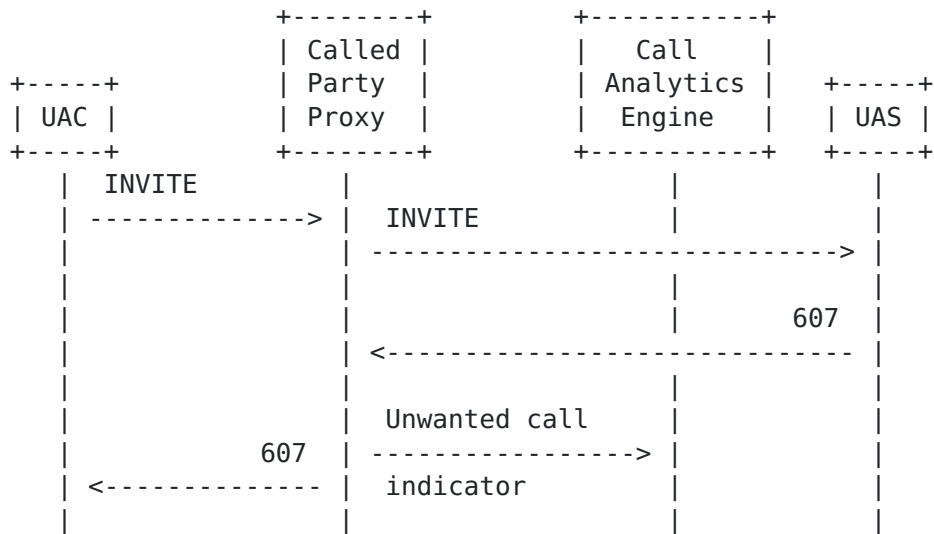
Figure 2: Unwanted (607) Ladder Diagram
