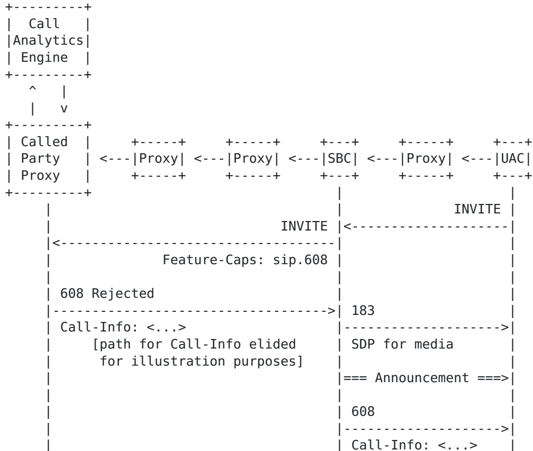
Figure 5: Legacy Operation
