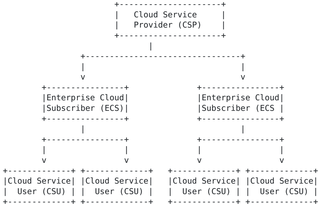
Figure 1: SCIM Actors
