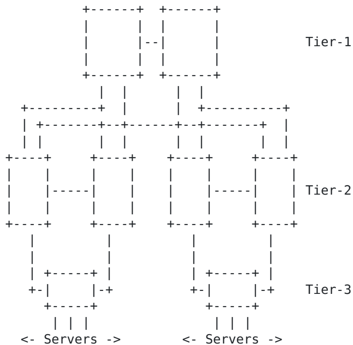
Figure 1: Typical DC network topology
