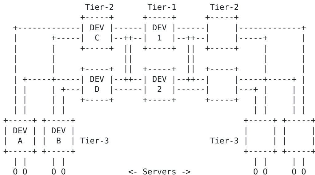
Figure 6: 5-Stage Clos topology
