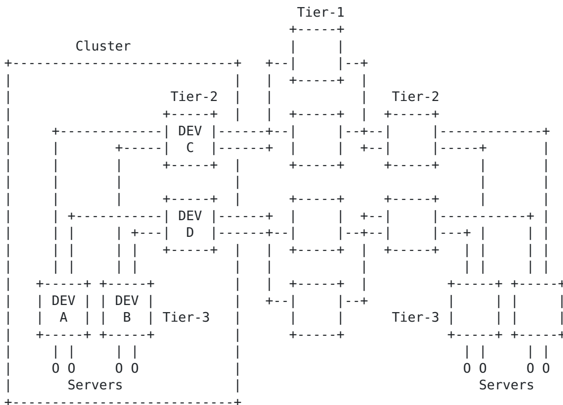
Figure 3: 5-Stage Clos topology
