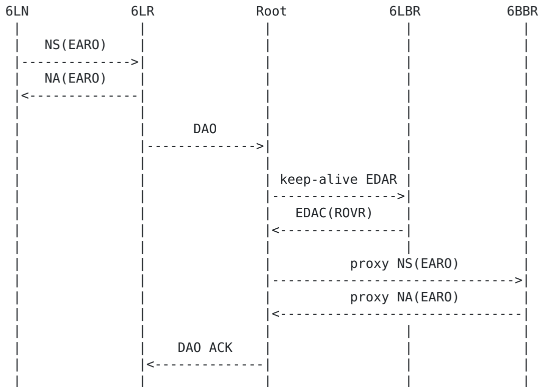
Figure 3: Next Registration Flow
