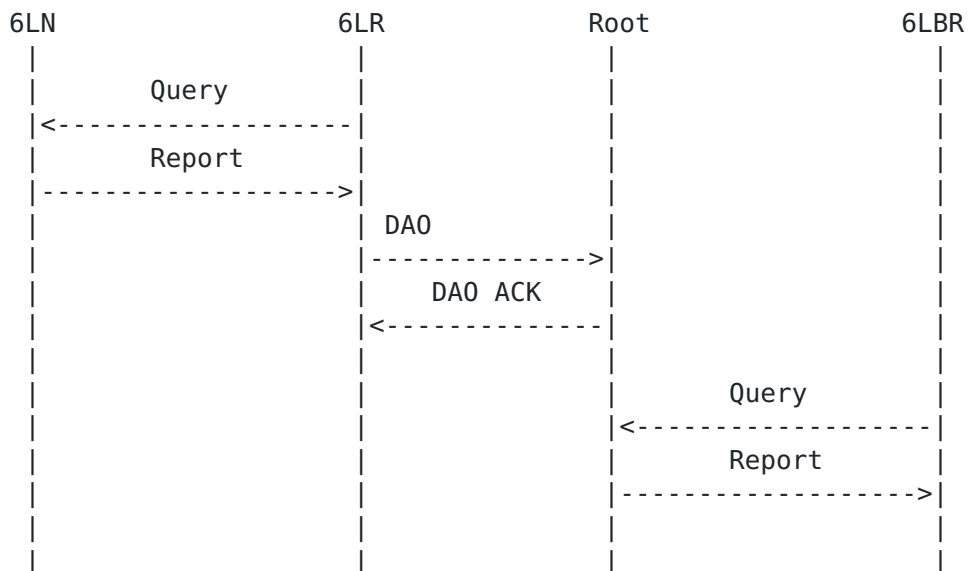
Figure 5: Next Registration Flow
