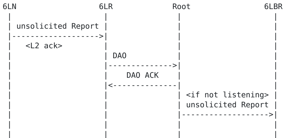
Figure 4: First Multicast Registration Flow
