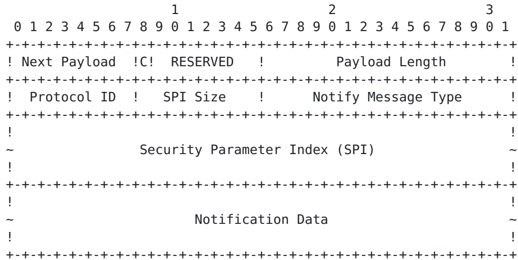
Figure 1. Notify Payload format.
