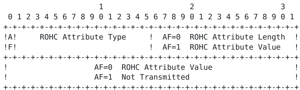
Figure 2. Format of the ROHC Attribute.
