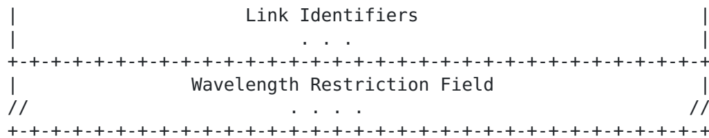
Figure 4 Wavelength Restriction Constraint TLV Encoding
