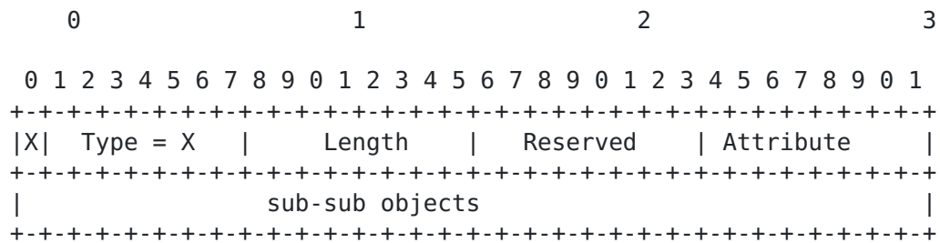
Figure 5 Signaling Processing XR0 Sub-Object
