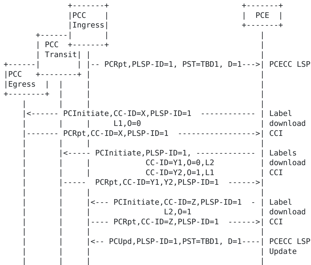
Figure 2: Basic PCECC LSP setup
