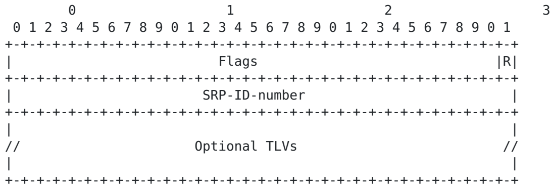
Figure 2: The SRP Object format
