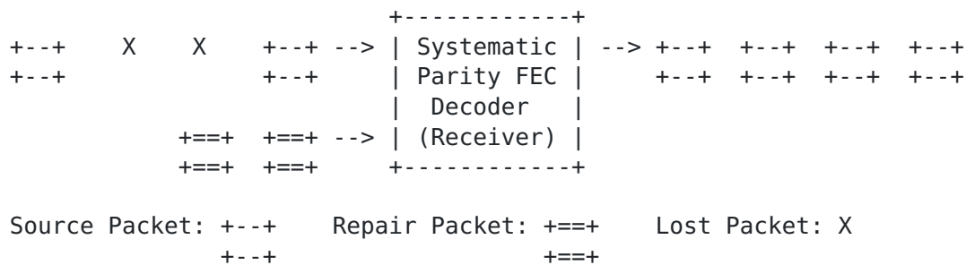
Figure 2: Block diagram for systematic parity FEC decoder
