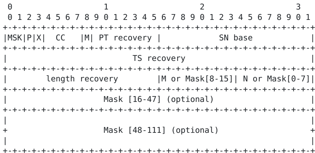
Figure 10: Format of the FEC header
