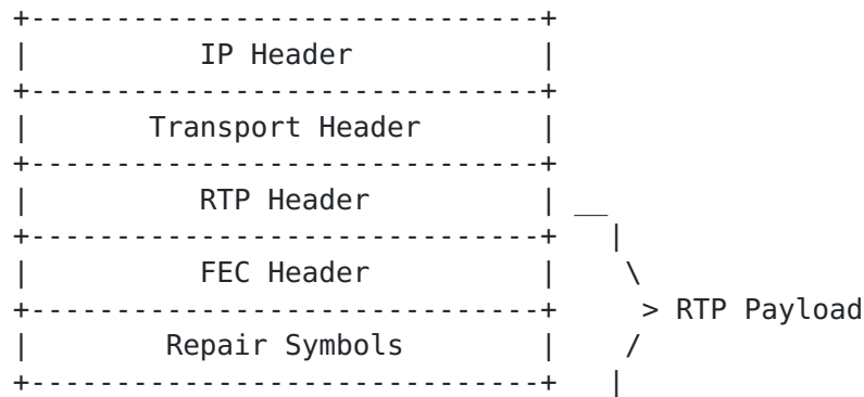
Figure 9: Format of repair packets
