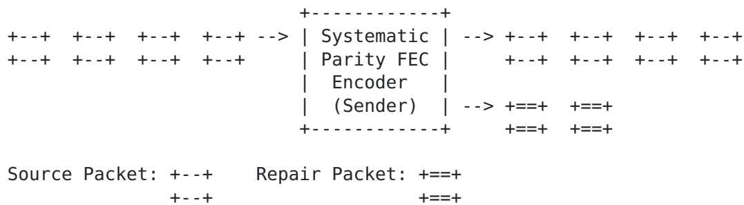
Figure 1: Block diagram for systematic parity FEC encoder
