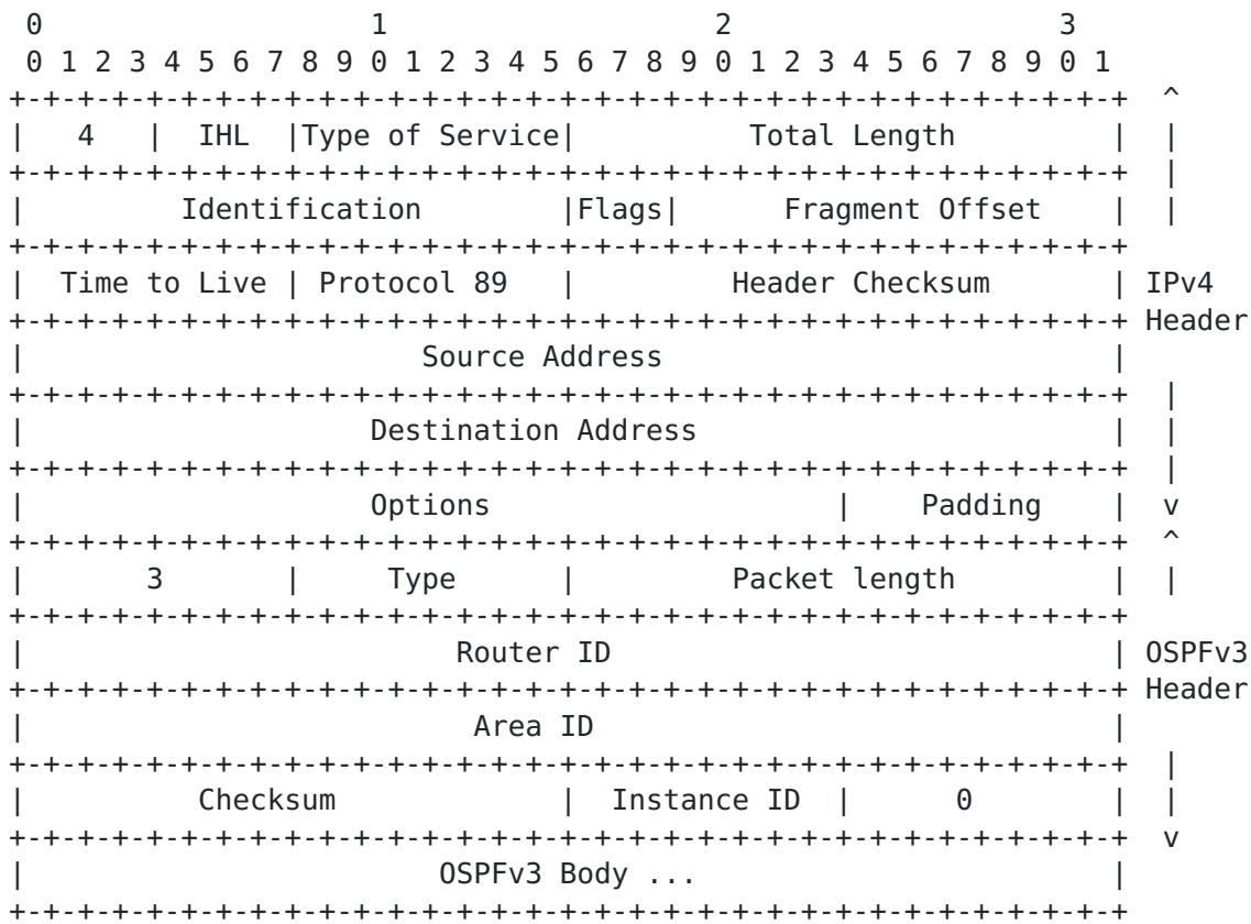
Figure 1: An IPv4 packet encapsulating an OSPFv3 packet.
