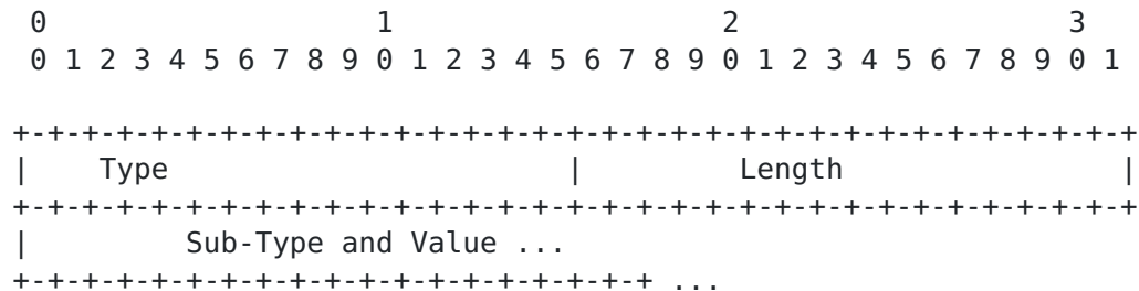
Figure 2: Link MSD Sub-TLV
