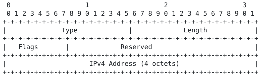
IPv4 Backup ER0 Sub-TLV format
