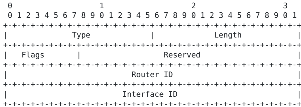
Unnumbered Interface ID Backup ERO Sub-TLV format
