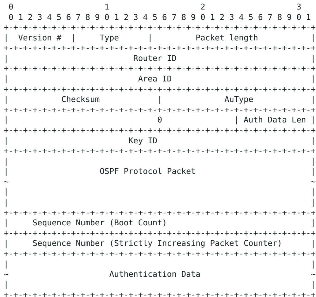
Figure 1 - Extended Sequence Number Packet Extensions
