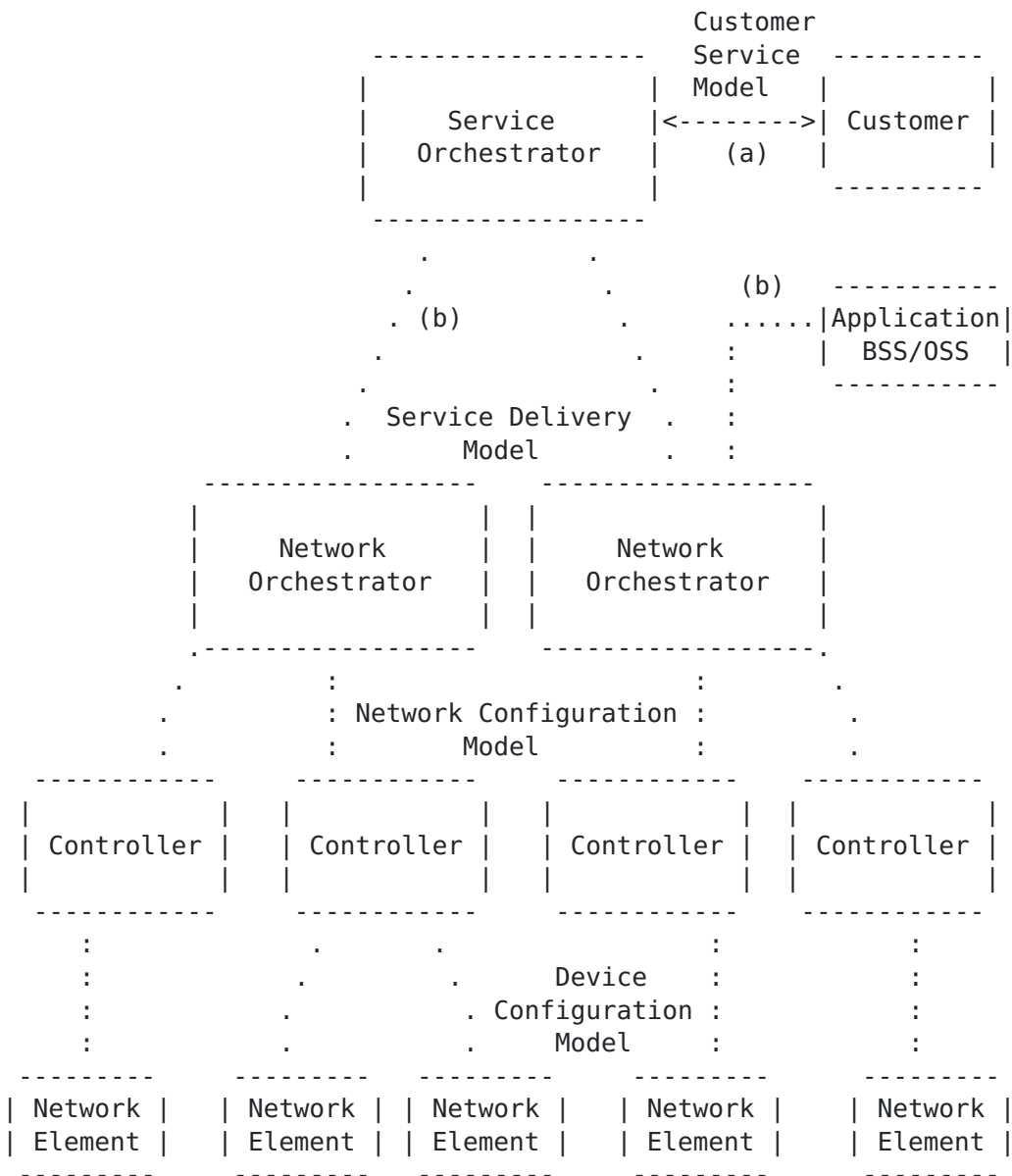
Figure 3: An Example SDN Architecture with a Service Orchestrator
