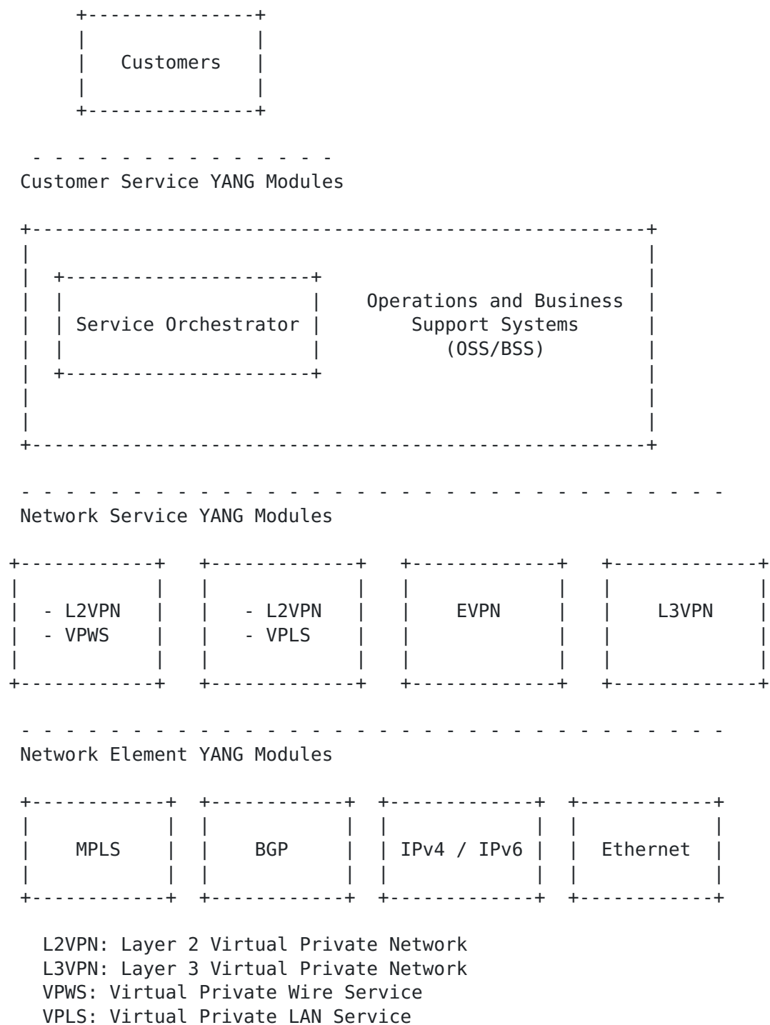
Figure 4: YANG Module Layers Showing Service Models
