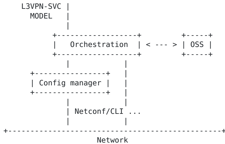
Figure 5: The L3SM Service Architecture
