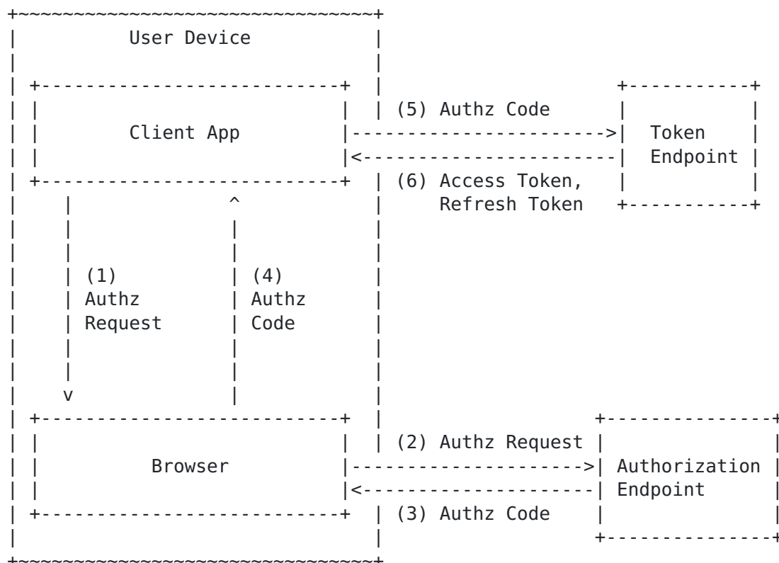
Figure 1: Native App Authorization via External User-agent
