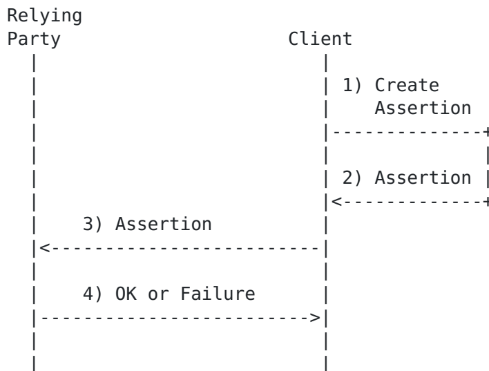
Figure 2: Self-Issued Assertion
