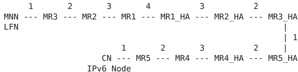
Figure 8: MNN and CN are standard IPv6 nodes
