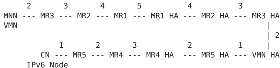
Figure 10: MNN is a MIPv6 mobile node and CN is a standard IPv6 node
