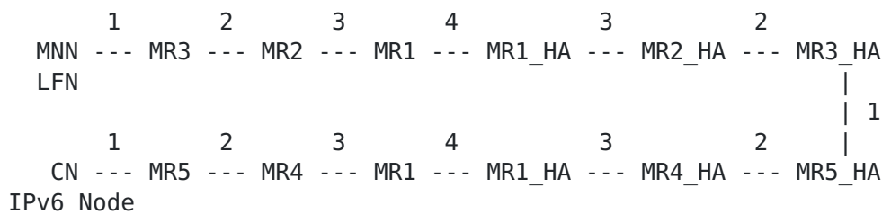
Figure 12: MNN and CN are standard IPv6 nodes
