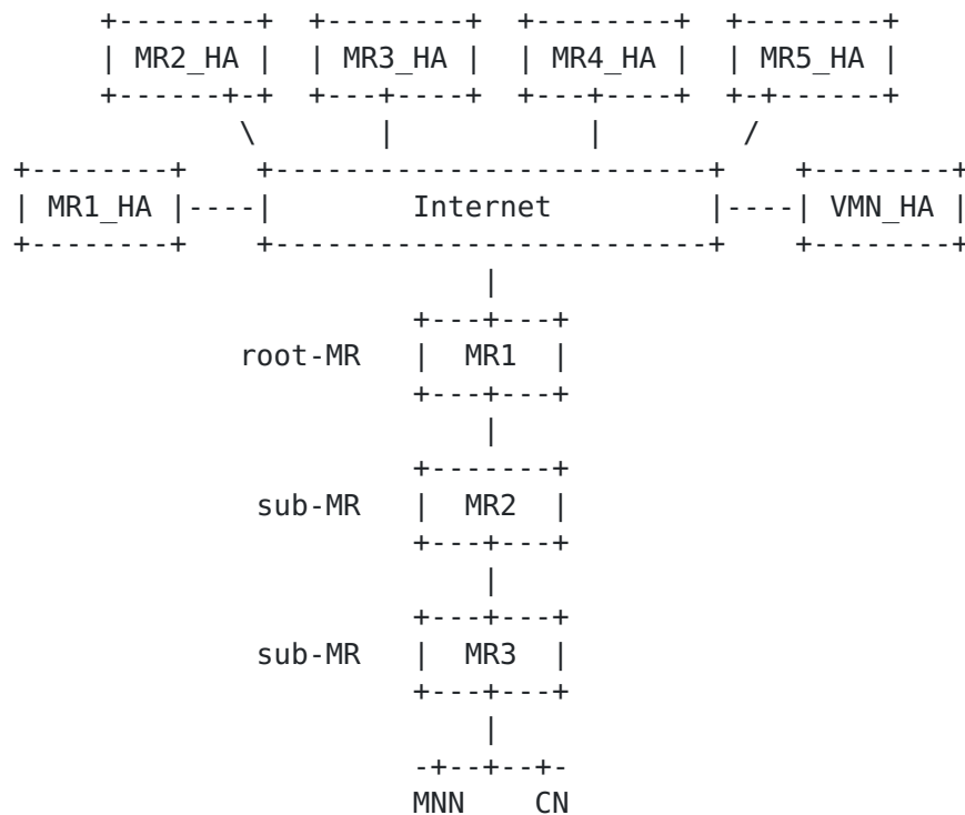
Figure 15: MNN and CN located behind the same nested MR
