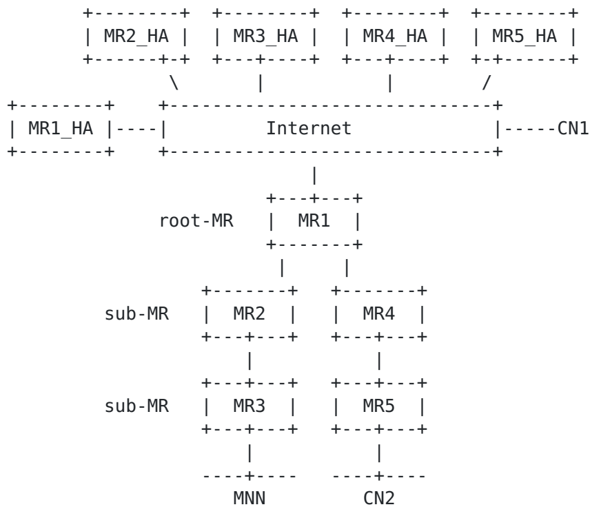
Figure 1: An example of nested Mobile Network
