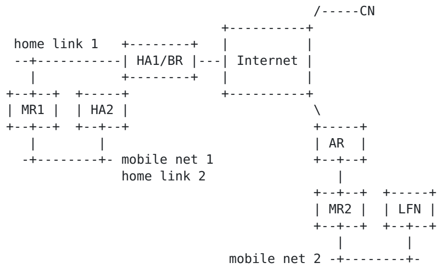
Figure 20: Mobile Network 2 Leaves Home
