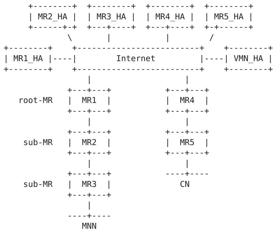
Figure 7: MNN and CN located in distinct nested NEMOs
