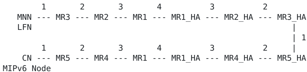
Figure 13: MNN and CN are MIPv6 mobile nodes
