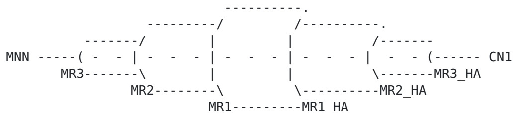
Figure 2: Nesting of Bi-Directional Tunnels
