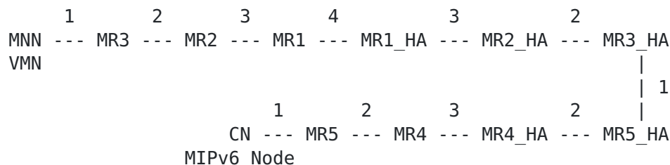
Figure 9: MNN and CN are MIPv6 mobile nodes
