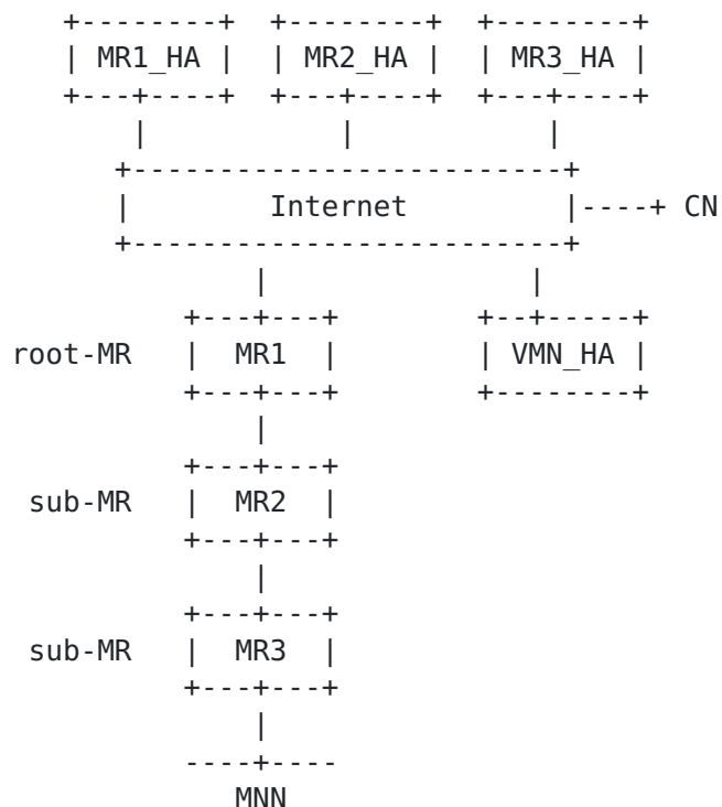
Figure 3: CN located at the infrastructure
