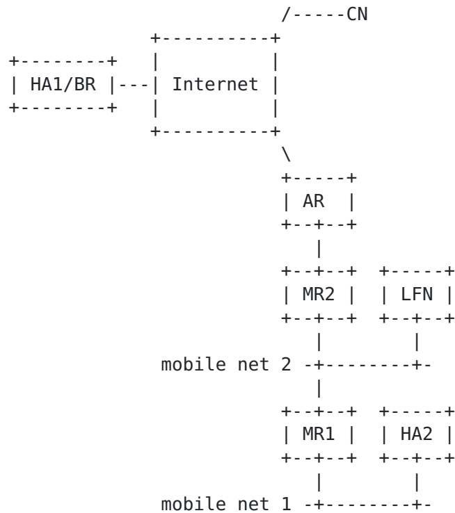
Figure 21: Stalemate Situation Occurs
