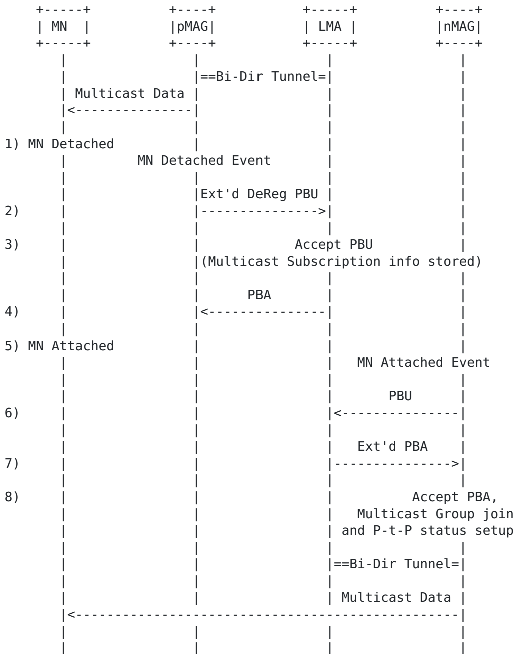
Figure 4: Proactive handover
