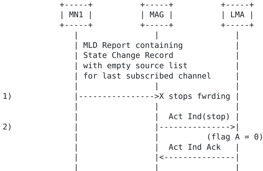
Figure 3: Multicast Activity set to OFF
