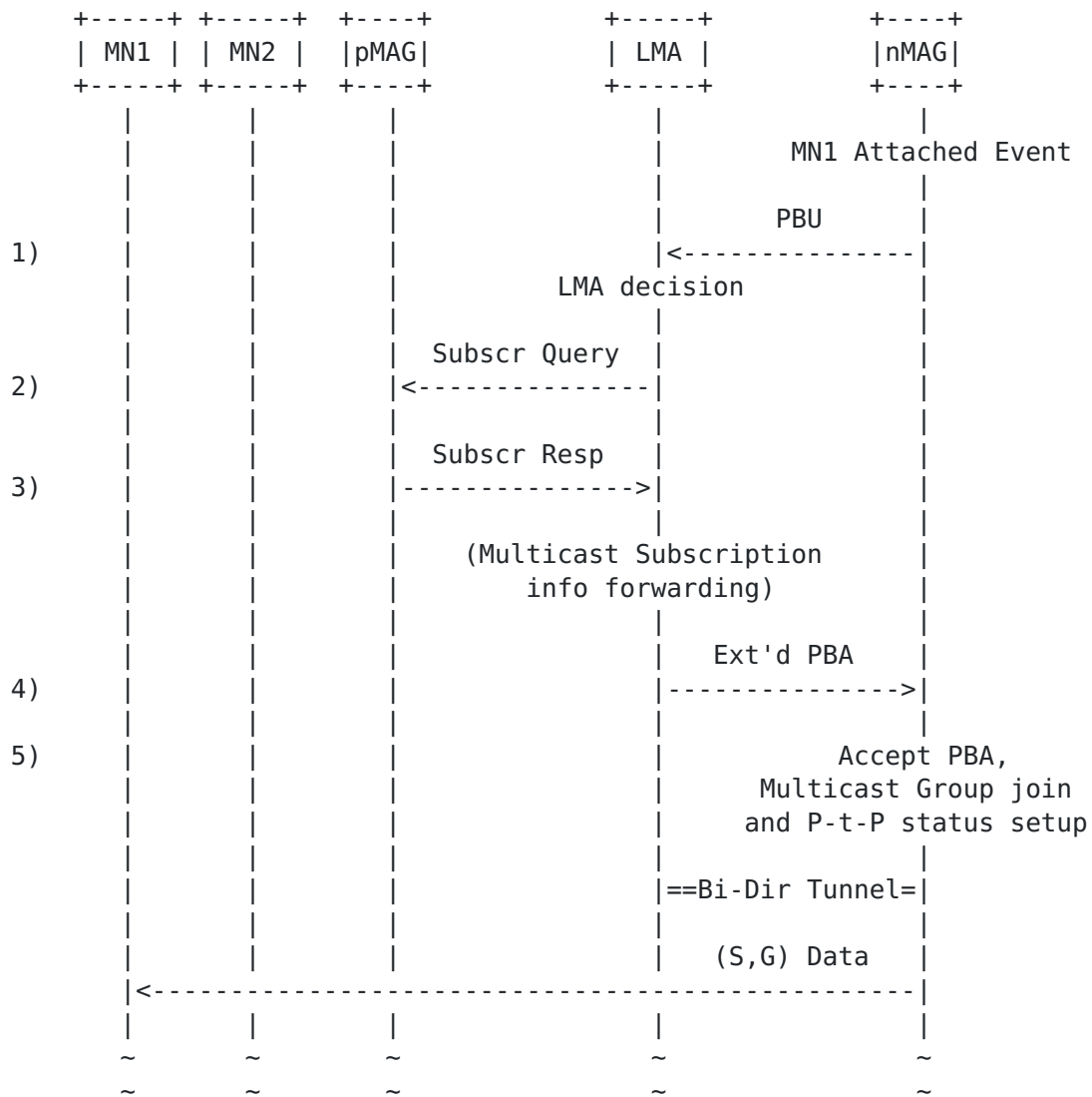
Figure 5: Reactive handover (steps 1 to 5)
