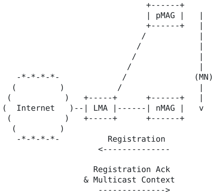
Figure 1: High level solution description
