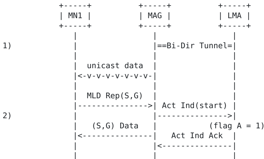
Figure 2: Multicast Activity set to ON
