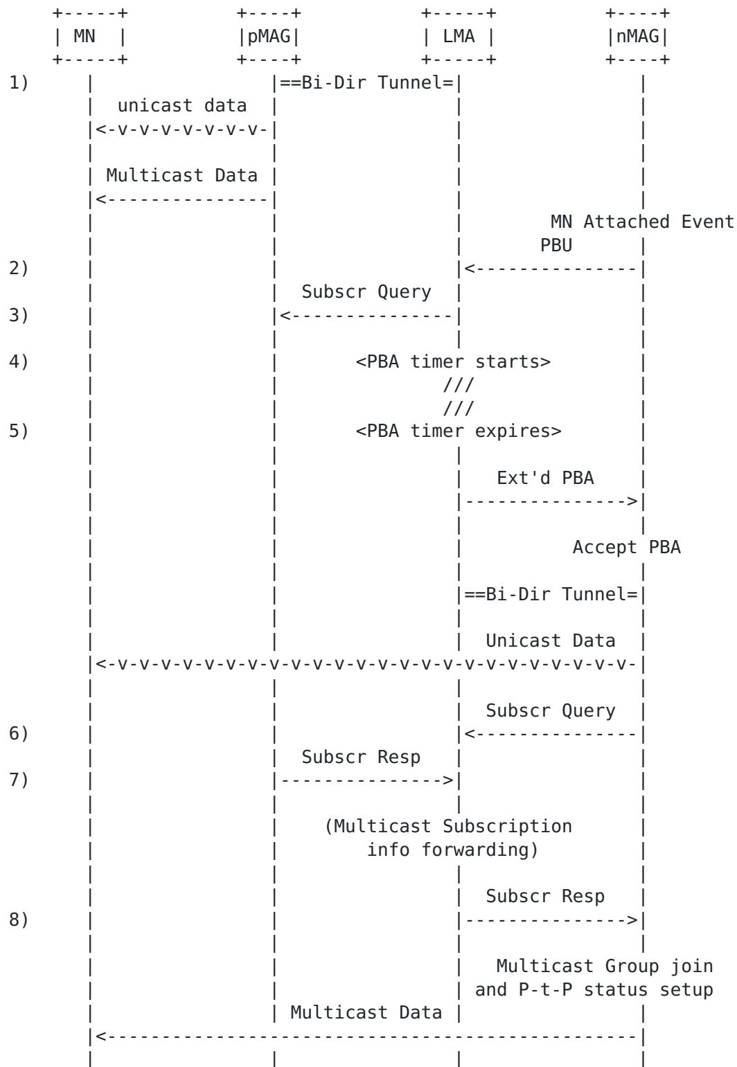
Figure 10: Decoupling of unicast and multicast signaling
