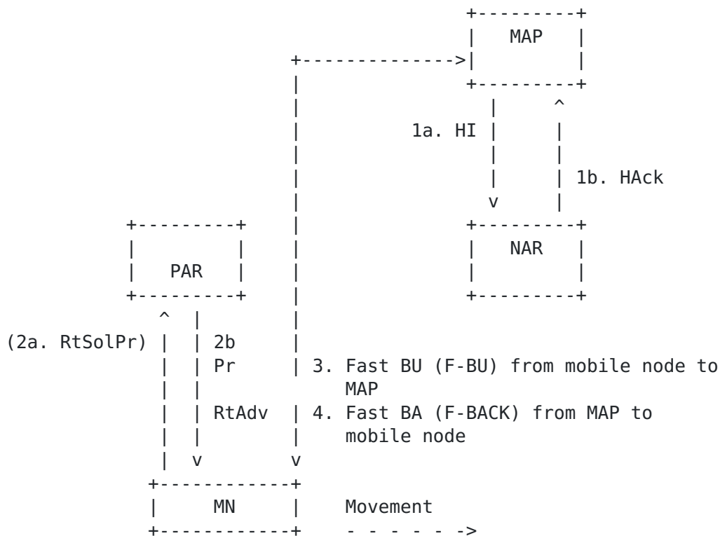
Figure A.2 Fast Mobile IPv6 Handover Protocol using HMIPv6
