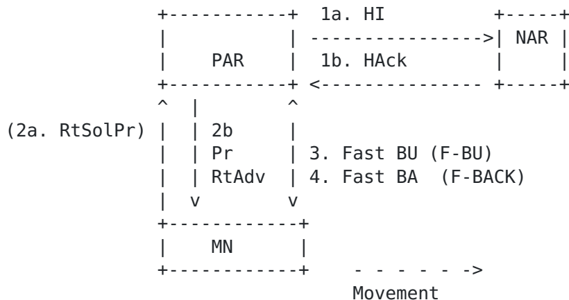
Figure A.1 - Fast Mobile IPv6 Handover Protocol
