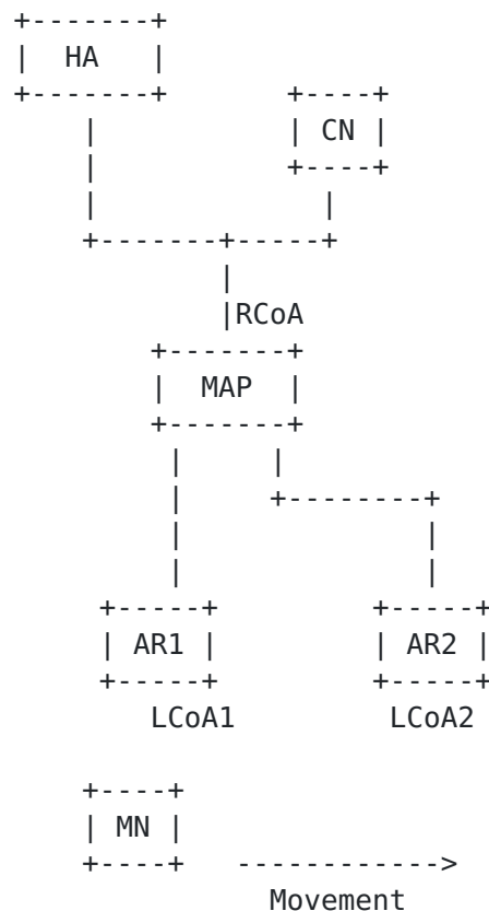
Figure 1: Hierarchical Mobile IPv6 domain
