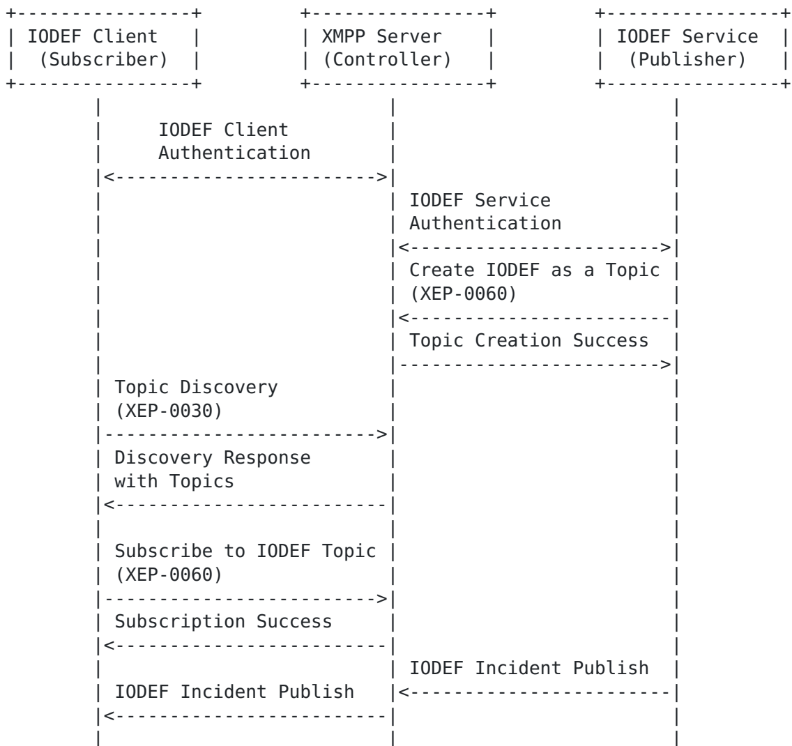
Figure 2: IODEF Example Workflow
