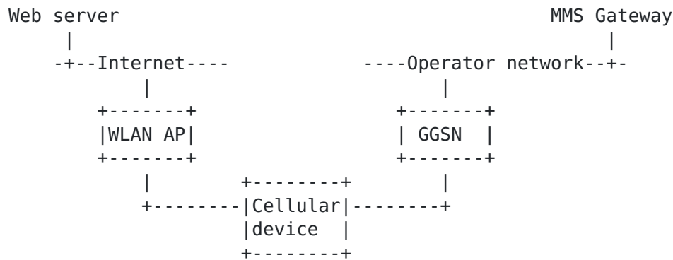
A cellular device with two network interfaces
