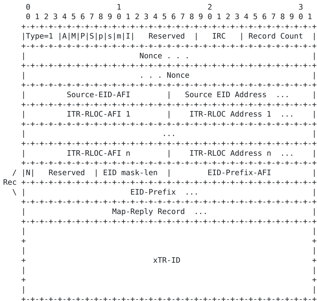
Figure 1: Map-Request with N-bit and xTR-ID
