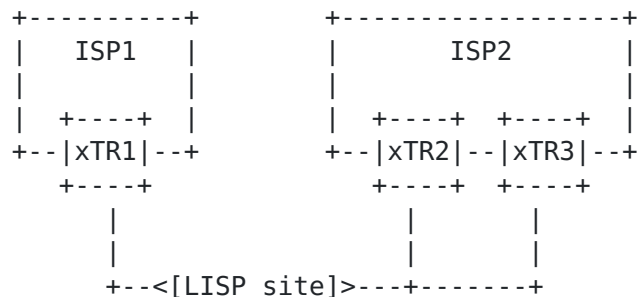
Figure 2: xTR at the PE
