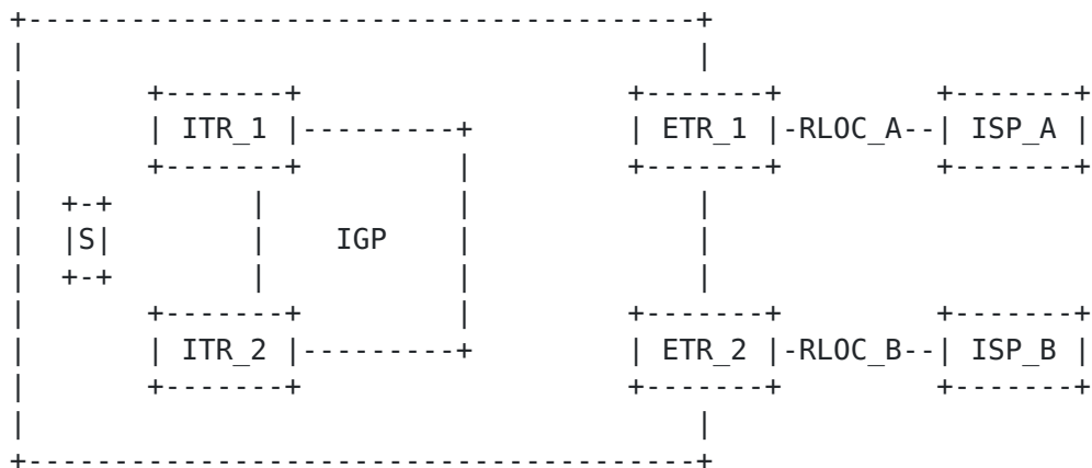
Figure 5: Split ITR/ETR Scenario
