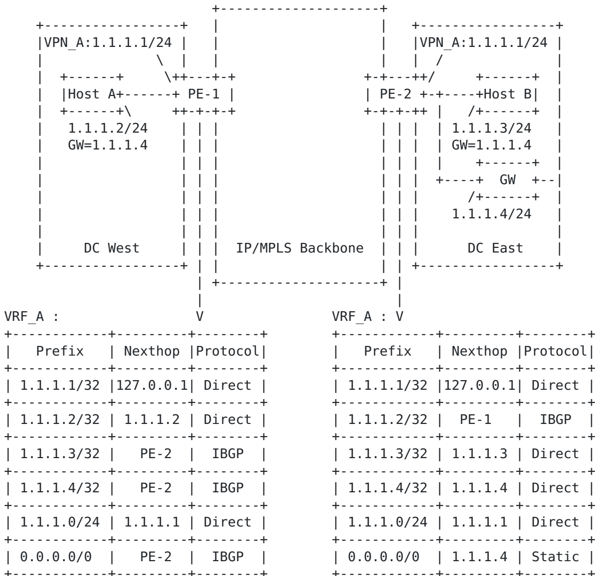
Figure 2: Inter-subnet Unicast Example (1)
