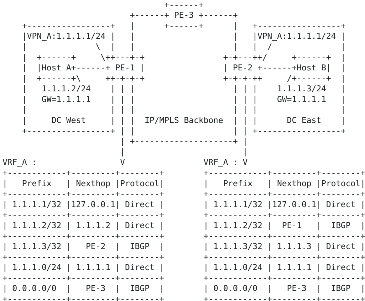
Figure 4: Inter-subnet Unicast Example (3)
