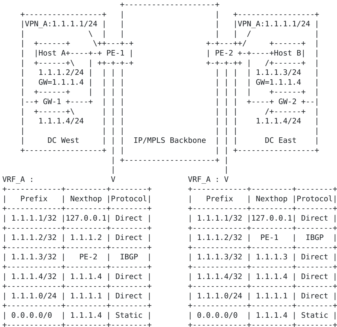
Figure 3: Inter-subnet Unicast Example (2)
