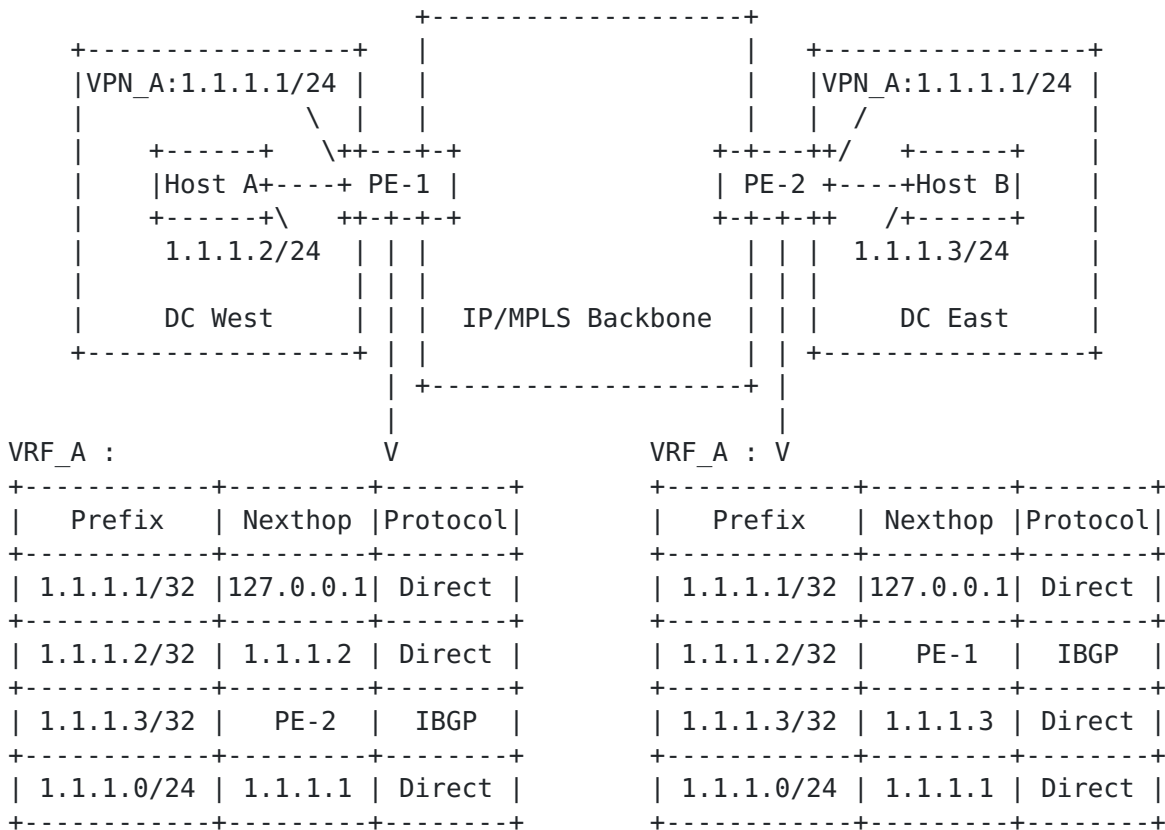
Figure 1: Intra-subnet Unicast Example
